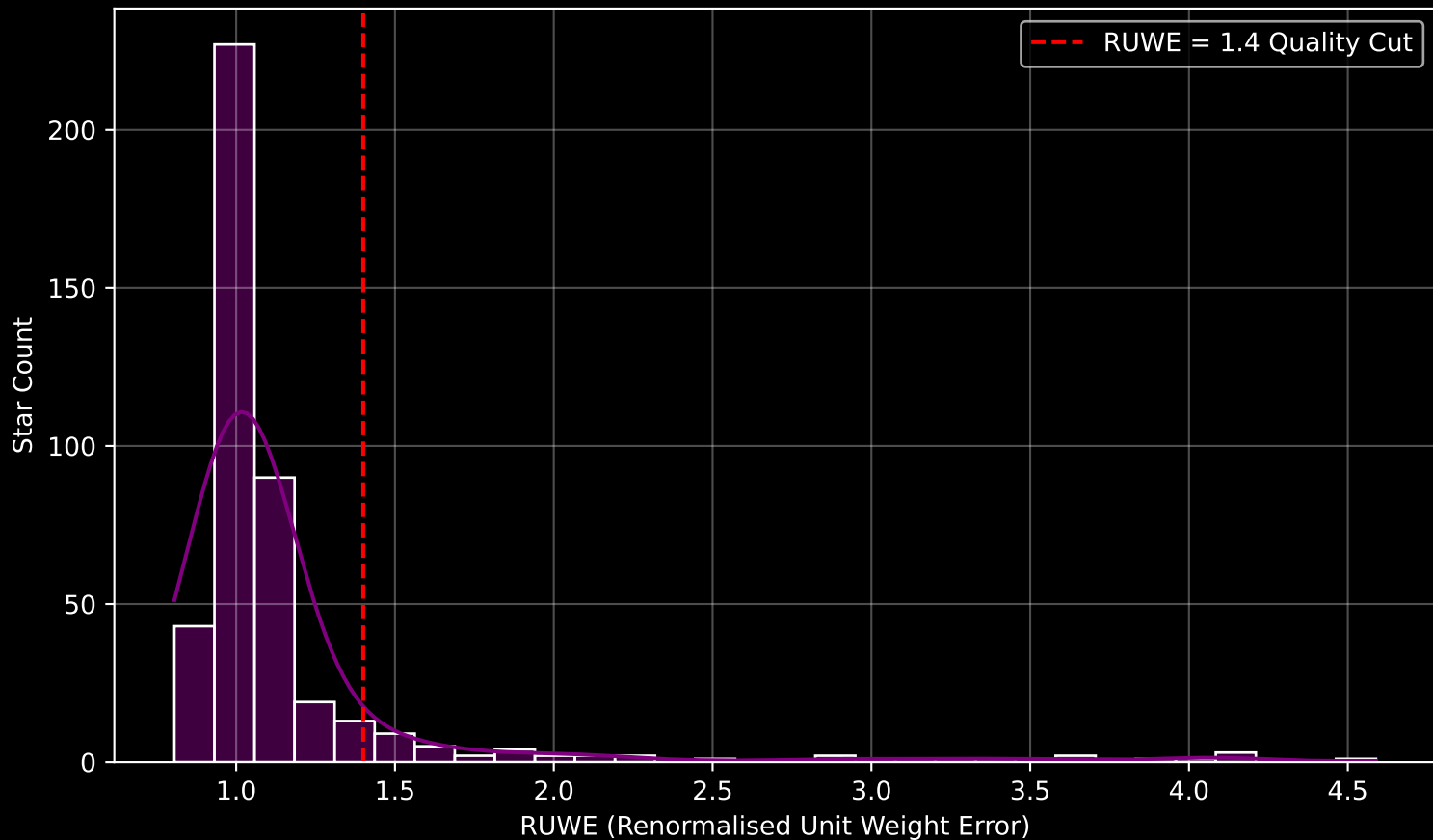
GAPOGEE DR17 Field [N188] RUWE Distribution (n= 433)
