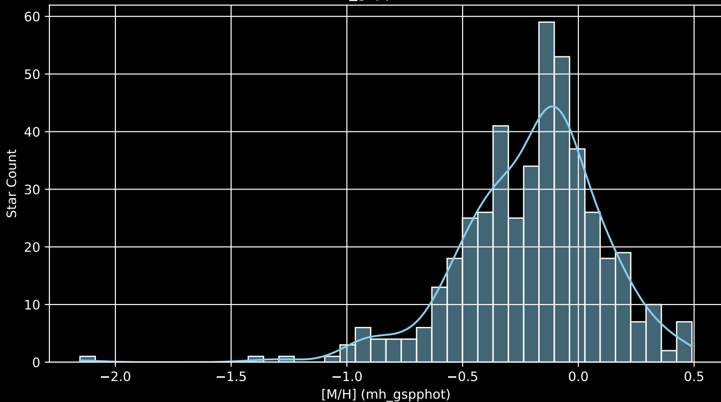
APOGEE DR17 Field: [N188 [M/H] (mh_gspphot) (n= 451)
