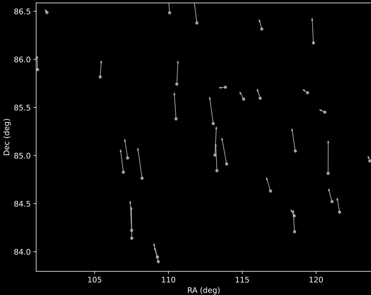
APOGEE DR17 Cluster 15 Proper Motion Vectors (n=33)
