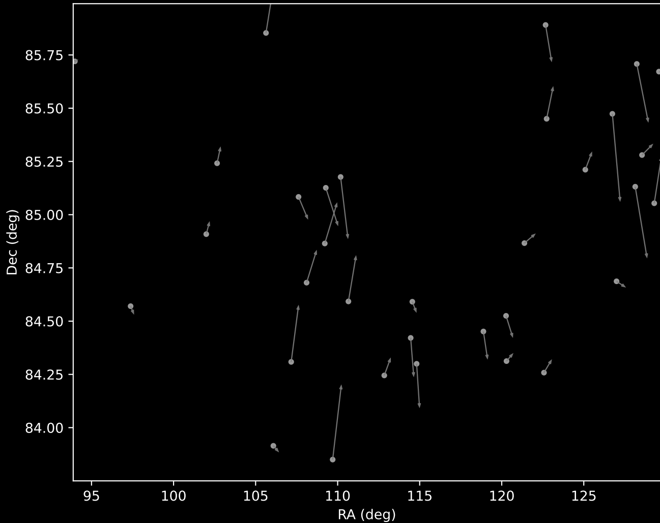
APOGEE DR17 Cluster 14 Proper Motion Vectors (n=33)
