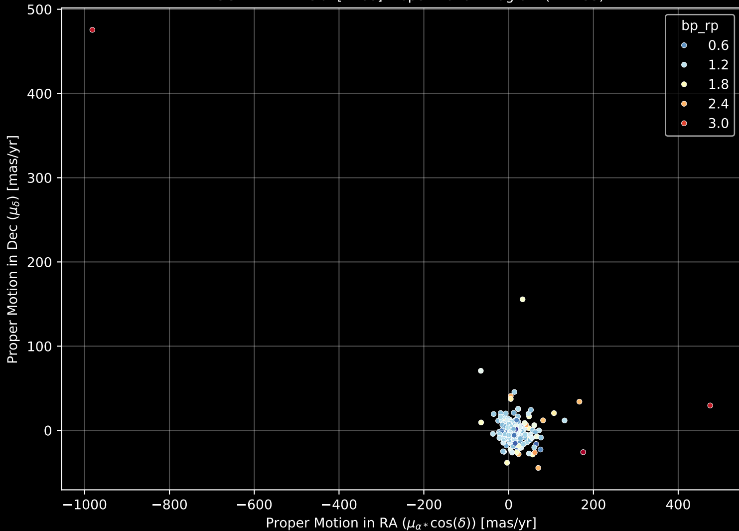
APOGEE DR17 Field: [N188] Proper Motion Diagram (n= 455)
