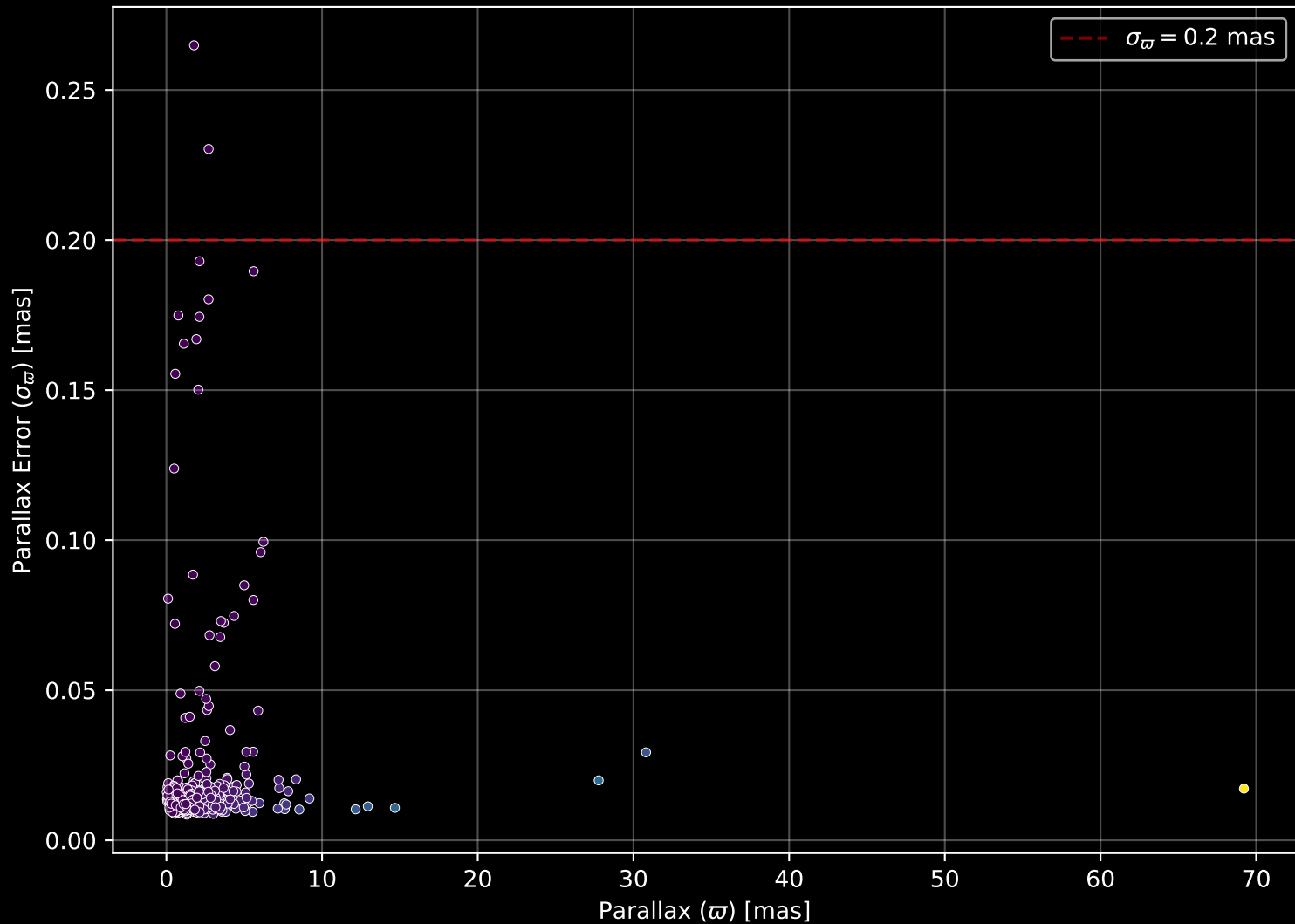
APOGEE DR17 Field: [N188] Parallax Quality (n= 455)
