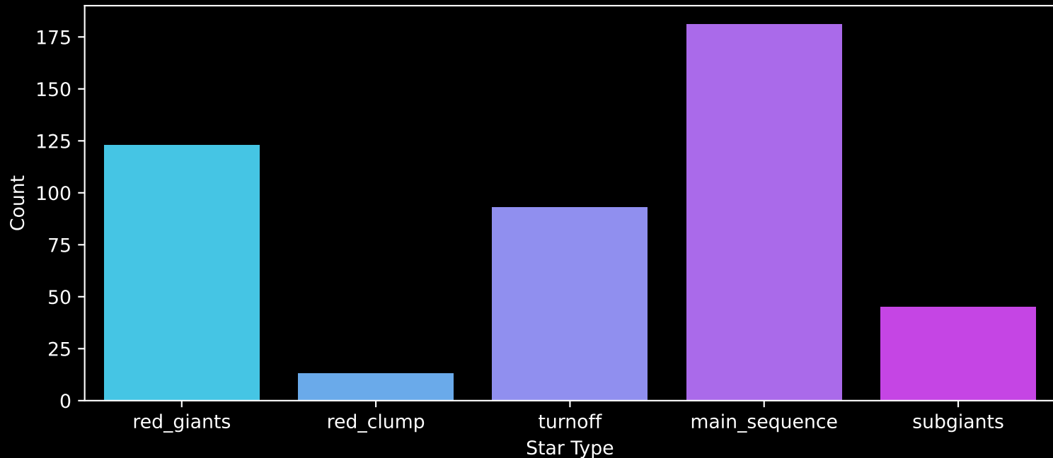
APOGEE DR17 Field: [N188] Count plot of Star Type
